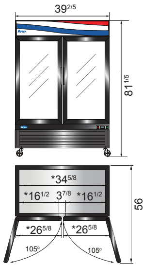
MCF8733GR
