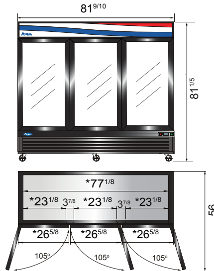
MCF8724GR
