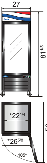
MCF8722GR
